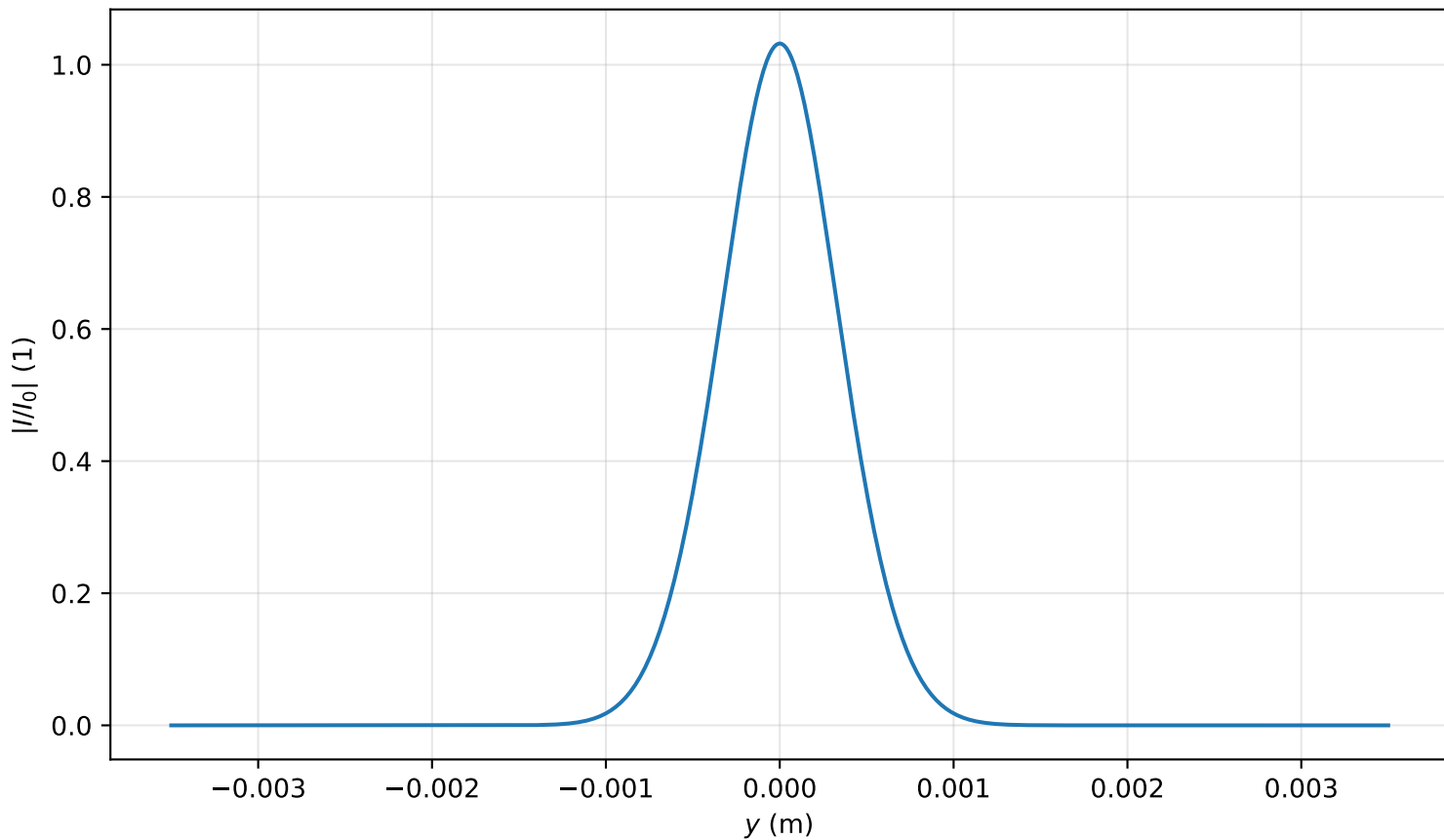
Intensity profile I(x=0, y, z=0.318)/I_0 , P_{in}=0.6P_{cr} , artificial time
